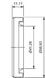
SECTION U-U
