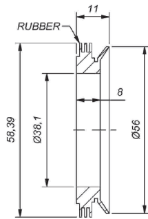
SECTION T-T
